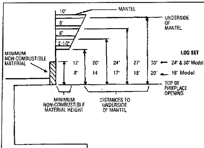
Minimum Mantel Clearance
