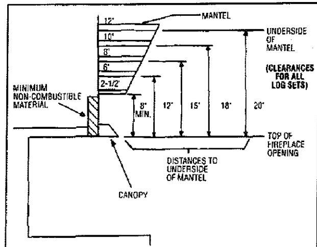
Minimum Mantel Clearance with Canopy
